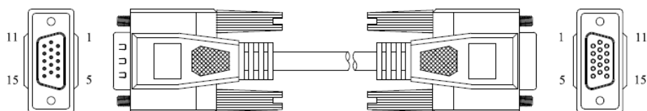
P1 HDB15M
